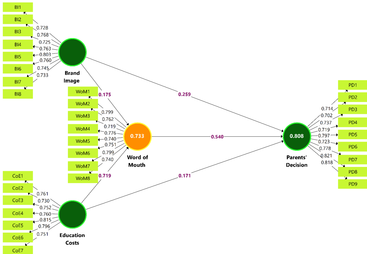
Gambar 1. PLS – ALGORITM
