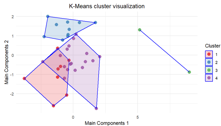
Figure. 2. Visualization of GII Clustering based on the K-Means Algorithm Development of GII in Indonesia
